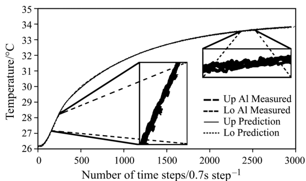
Fig. 3 Center-A1 interface temperature predictions and measurements for redwood flooring specimen (14% moisture content)
