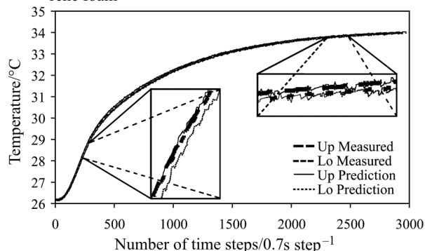
Fig. 2 Center-sensor interface temperature predictions and measurements for redwood flooring specimen (3% moisture content)
